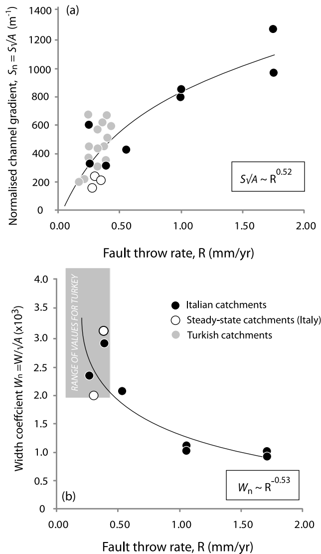
Figure 8. (a) Drainage area normalized channel slope, S_n = S\sqrt{A} against fault throw rate, R . White circles represent channel gradients at the fault for catchments that have reached topographic steady state. Where the transient wave of incision had migrated more than 2 km upstream of the fault, we used the local knickzone gradient within 2 km of the knick-points indicated by stars in Figure 4. Line shows best fit power law dependence of S_n on R . (b) Mean knickzone channel width, W_n , normalized for drainage area at the fault, against fault throw rate, R , for Italy (points) and Turkey (box shows data range). Line shows best fit power law dependence of W_n on R .
